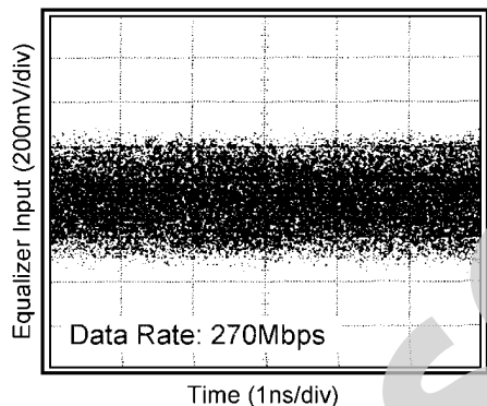
Before Equalization: 200m of Belden 8281 Coaxial Cable
