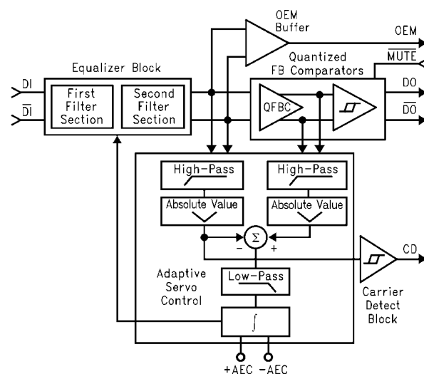
FIGURE 2. CLC014 Block Diagram
