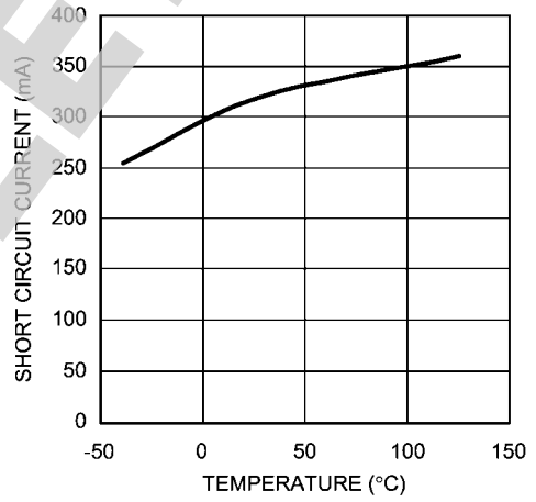
Short Circuit Current vs. Temperature ( V_{IN} = 3.3V )
