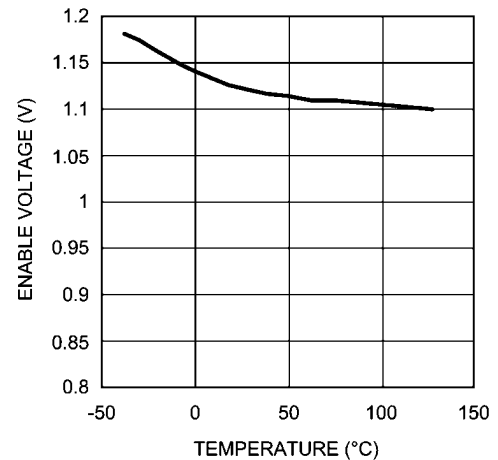
Enable Voltage vs. Temperature
