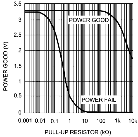
Power Good Pull-Up Resistor vs. Power Good
