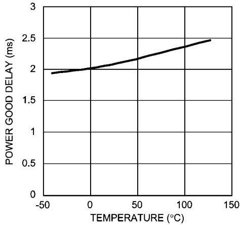
Power Good Delay vs. Temperature ( V_{IN} = 3.3V )
