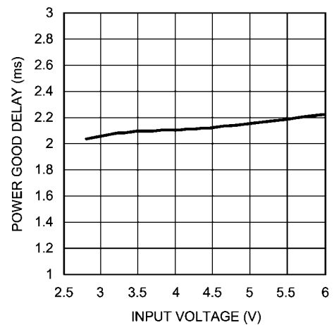
Power Good Delay vs. Input Voltage ( I_L = 100\mu A )
