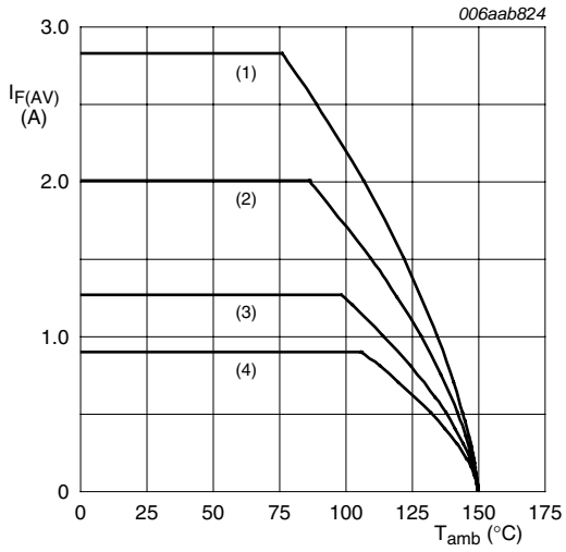
Ceramic PCB, Al_2O_3 , standard footprint T_j = 150\text{ }^{\circ}C (1) \delta = 1 ; DC (2) \delta = 0.5 ; f = 20 kHz (3) \delta = 0.2 ; f = 20 kHz (4) \delta = 0.1 ; f = 20 kHz
