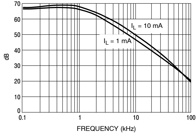
Figure 13. Ripple Rejection
