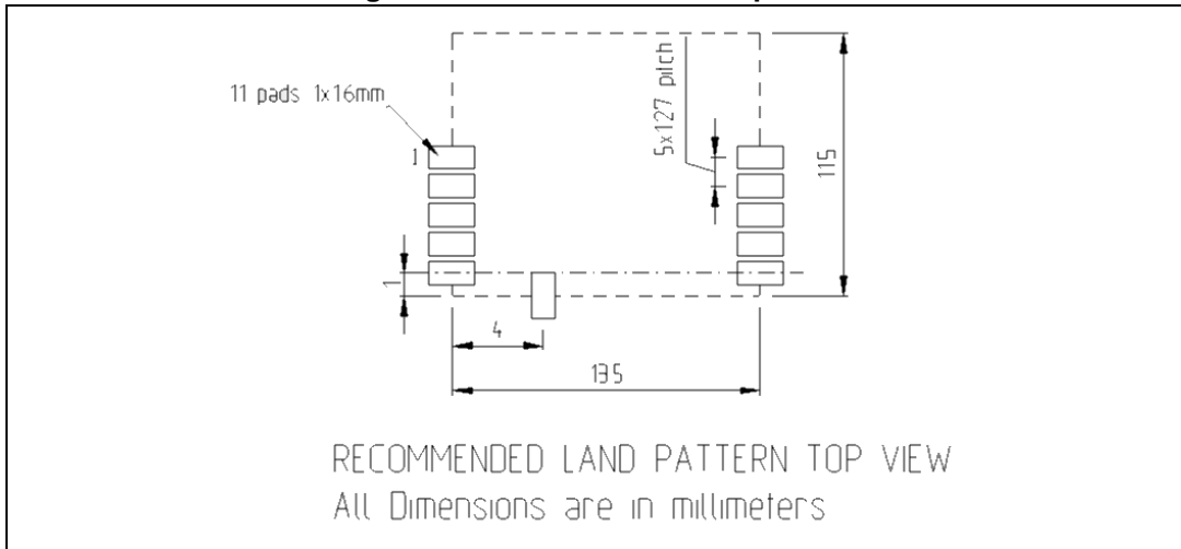
Figure 5. Recommended land pattern
