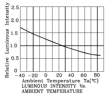
DERATING CURVE
