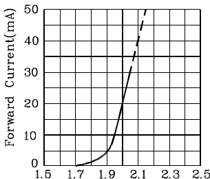
Forward Current(V) FORWARD CURRENT Vs FORWARD VOLTAGE
