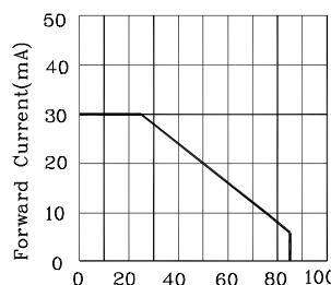
Ambient Temperature T_a(^{\circ}\text{C}) FORWARD CURRENT DERATING CURVE
