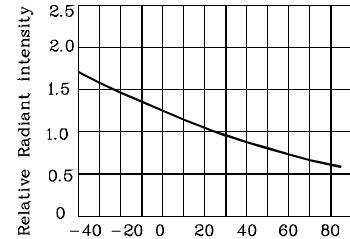
RADIANT INTENSITY Vs. AMBIENT TEMPERATURE
