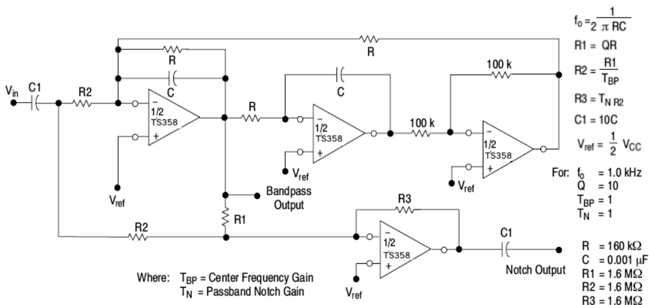
Figure 9. Bi-Quad Filter
