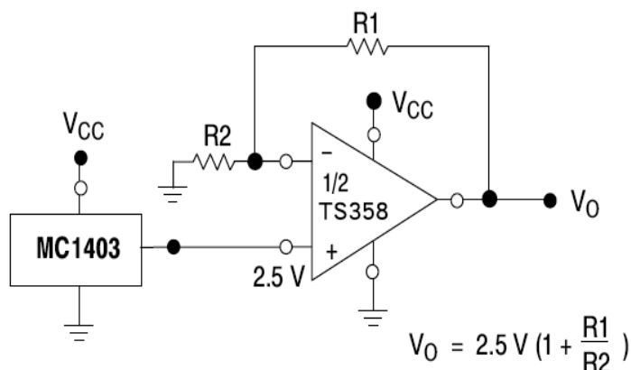
Figure 7. Voltage Reference
