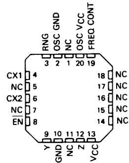
SN54LS624 . . . FK PACKAGE (TOP VIEW)
