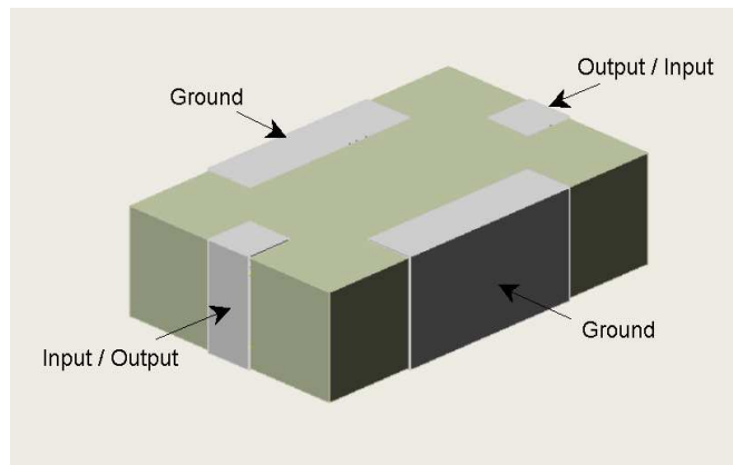
Fig 1. Outline of 2.4GHz Band Pass Filter 2012 size
