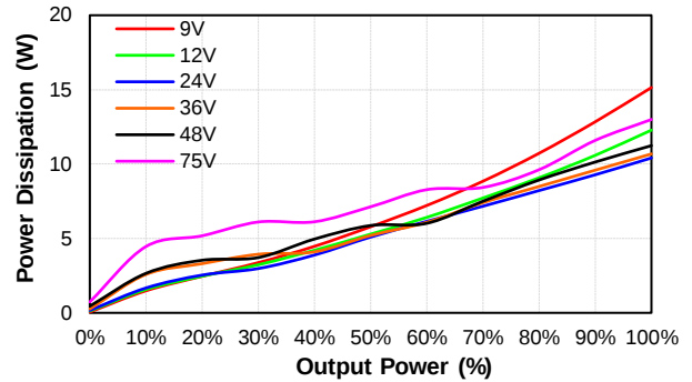
CQB100W8-36S24 Pd Vs Po @25 Deg. C
