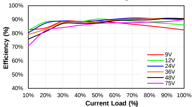
CQB100W8-36S05 Eff Vs Io @25 Deg. C
