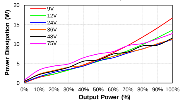
CQB100W8-36S15 Pd Vs Po @25 Deg. C
