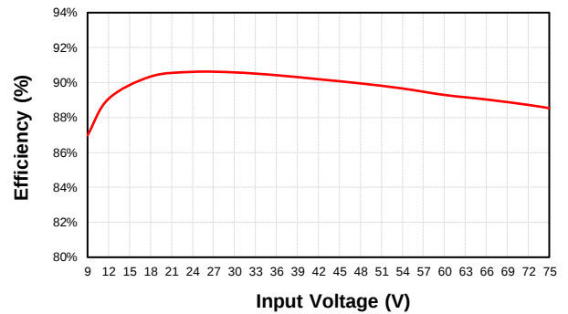
CQB100W8-36S24 Eff Vs Vin @25 Deg. C
