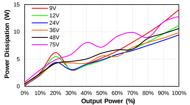
CQB100W8-36S48 Pd Vs Po @25 Deg. C
