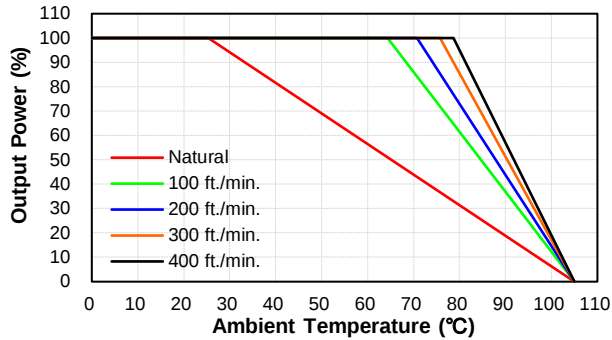
CQB100W8-36S28, 48, 54 Derating Curve with Heatsink QBT210 (Vin=36V)
