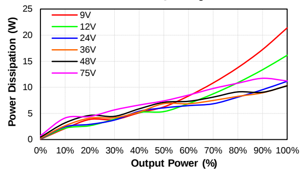
CQB100W8-36S05 Pd Vs Po @25 Deg. C
