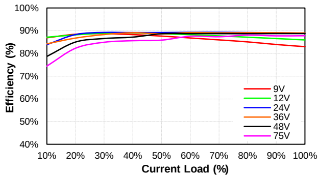
CQB100W8-36S12 Eff Vs Io @25 Deg. C
