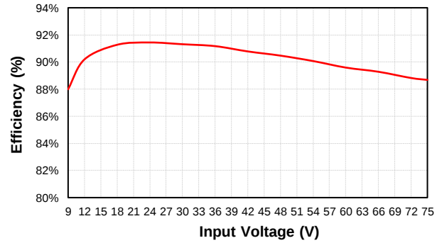
CQB100W8-36S48 Eff Vs Vin @25 Deg. C
