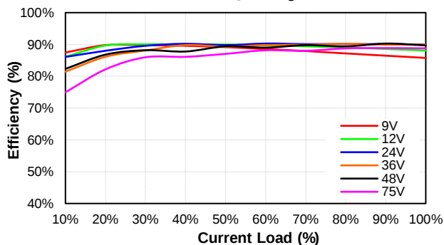
CQB100W8-36S15 Eff Vs Io @25 Deg. C
