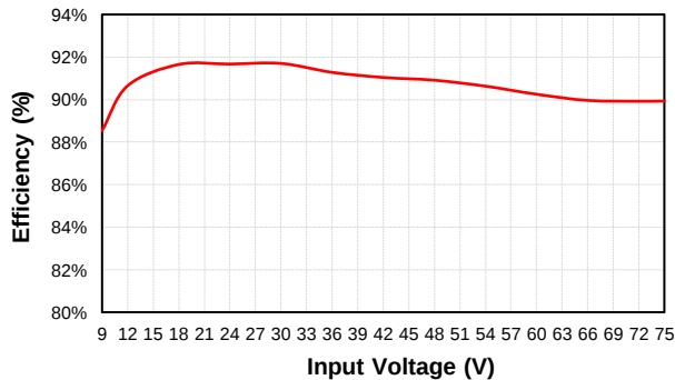
CQB100W8-36S54 Eff Vs Vin @25 Deg. C
