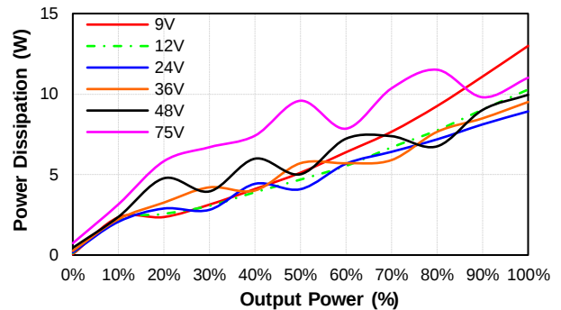
CQB100W8-36S54 Pd Vs Po @25 Deg. C
