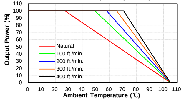
CQB150W14-72S05 Derating Curve with Heatsink QBL127 (Vin=72V)
