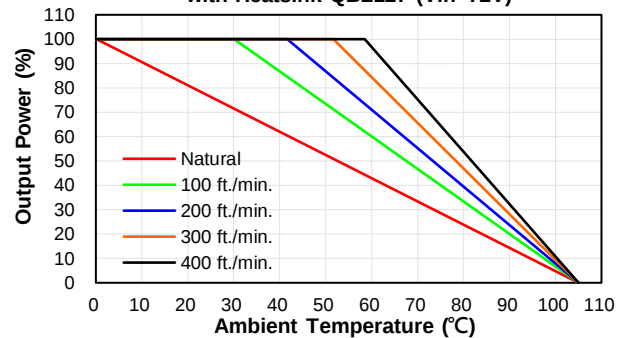
CQB150W14-72S24 Derating Curve with Heatsink QBL127 (Vin=72V)
