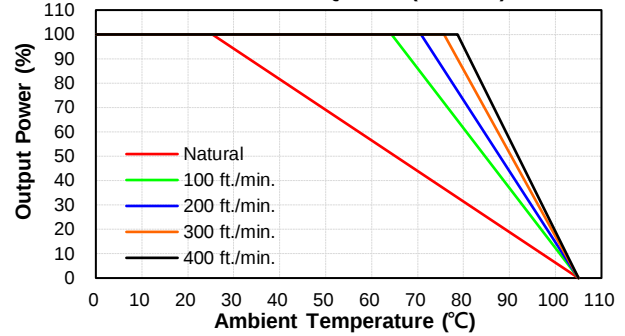
CQB150W14-72S12, 15, 28, 54 Derating Curve with Heatsink QBT210 (Vin=72V)
