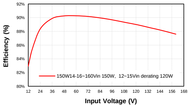
CQB150W14-72S28 Eff Vs Vin @25 Deg. C
