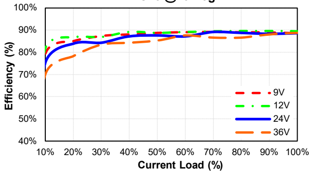
EC2SBW-24S15H Eff Vs Io @25 Deg. C
