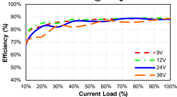
EC2SBW-24D15H Eff Vs Io @25 Deg. C
