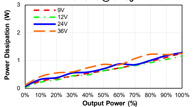
EC2SBW-24S15H Pd Vs Po @25 Deg. C
