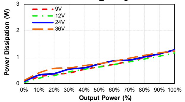
EC2SBW-24S12H Pd Vs Po @25 Deg. C
