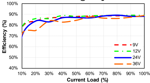
EC2SBW-24D12H Eff Vs Io @25 Deg. C
