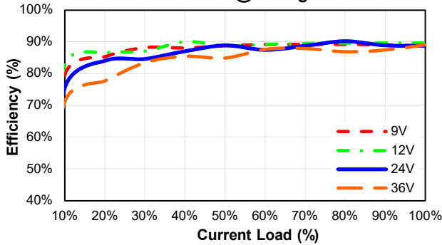
EC2SBW-24S12H Eff Vs Io @25 Deg. C
