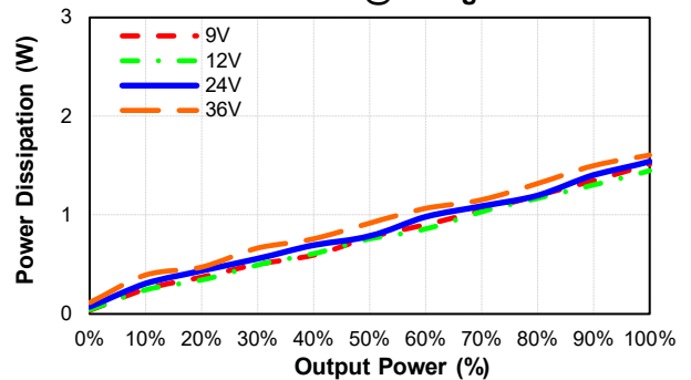
EC2SBW-24S33H Pd Vs Po @25 Deg. C
