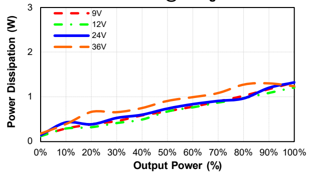
EC2SBW-24D12H Pd Vs Po @25 Deg. C
