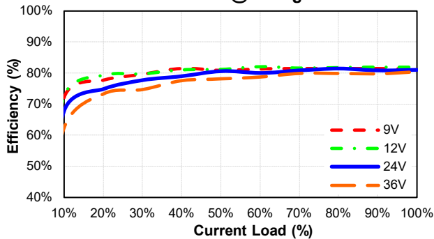
EC2SBW-24S33H Eff Vs Io @25 Deg. C
