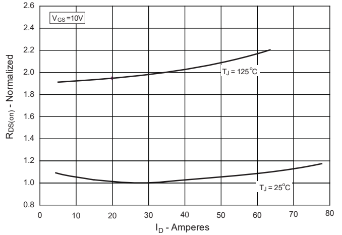
Fig. 4. R_{DS(on)} Normalized to I_D = 28\text{A} Value vs. Drain Current
