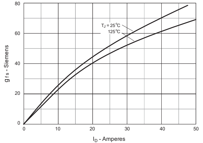
Fig. 6. Transconductance
