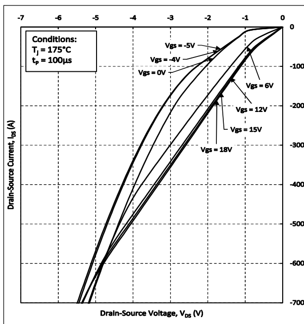
Figure 10. Freewheeling Diode Characteristics at T_J = 175^\circ\text{C}
