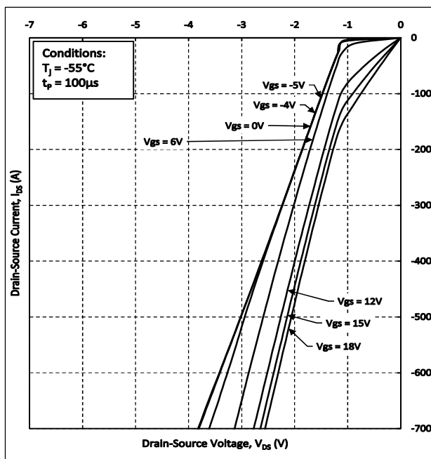
Figure 8. Freewheeling Diode Characteristics at T_J = -55^\circ\text{C}
