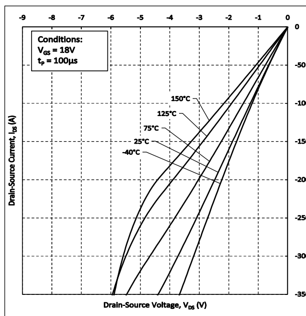
Figure 8. 3 rd Quadrant Characteristics at V_{GS} = 18V
